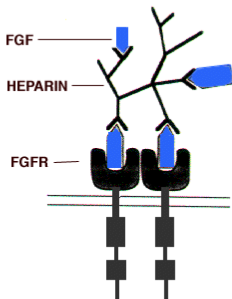
Figure 1 A model for heparin-induced dimerization and activation of the FGF receptors. (After Spivak-Kroizman et al., 1994).
